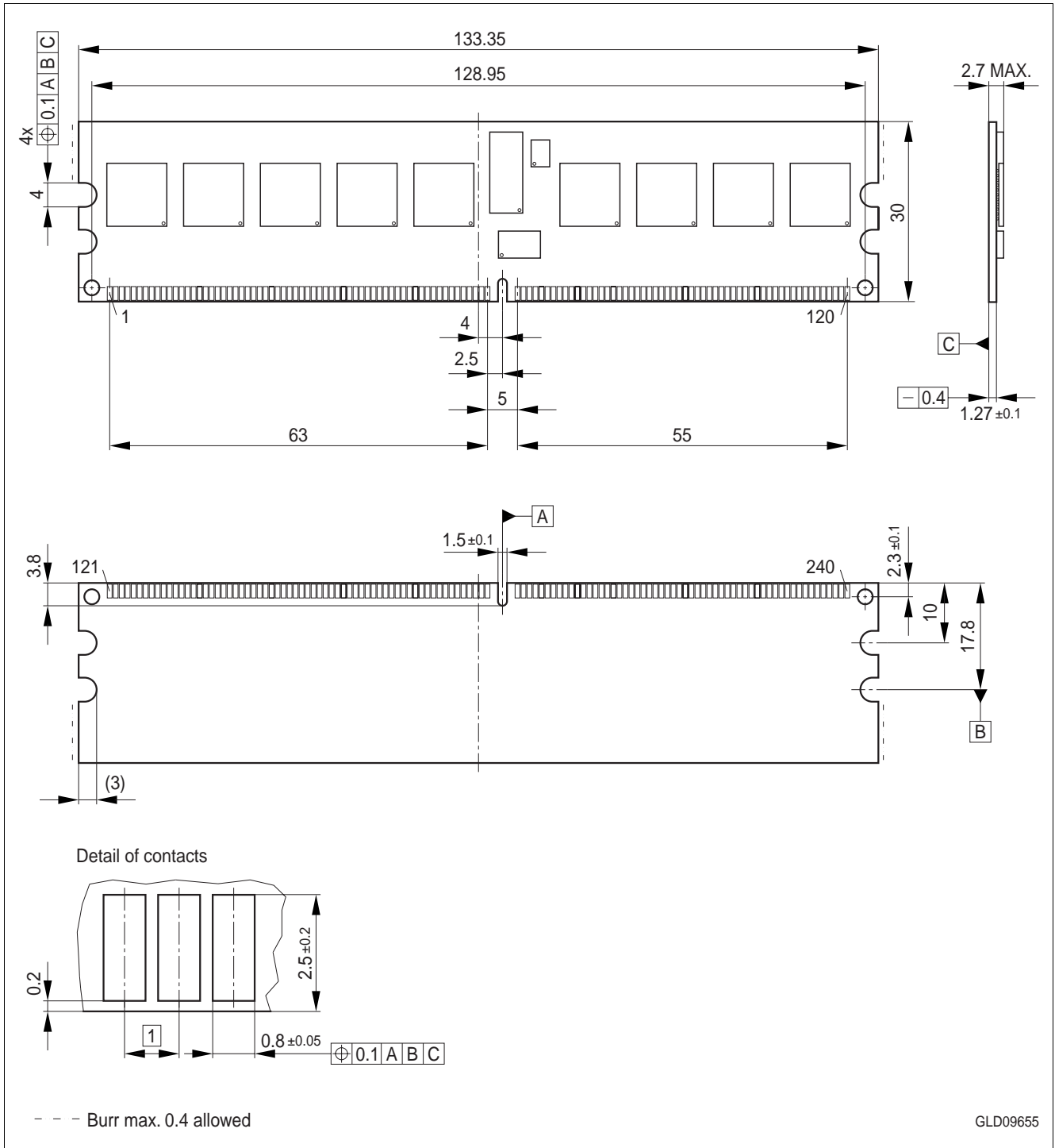
Figure 7 Package Outline Raw Card F L-DIM-240-11
