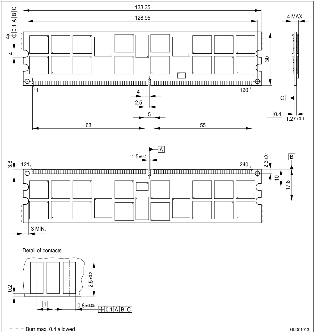
Figure 11 Package Outline Raw Card L L-DIM-240-40
