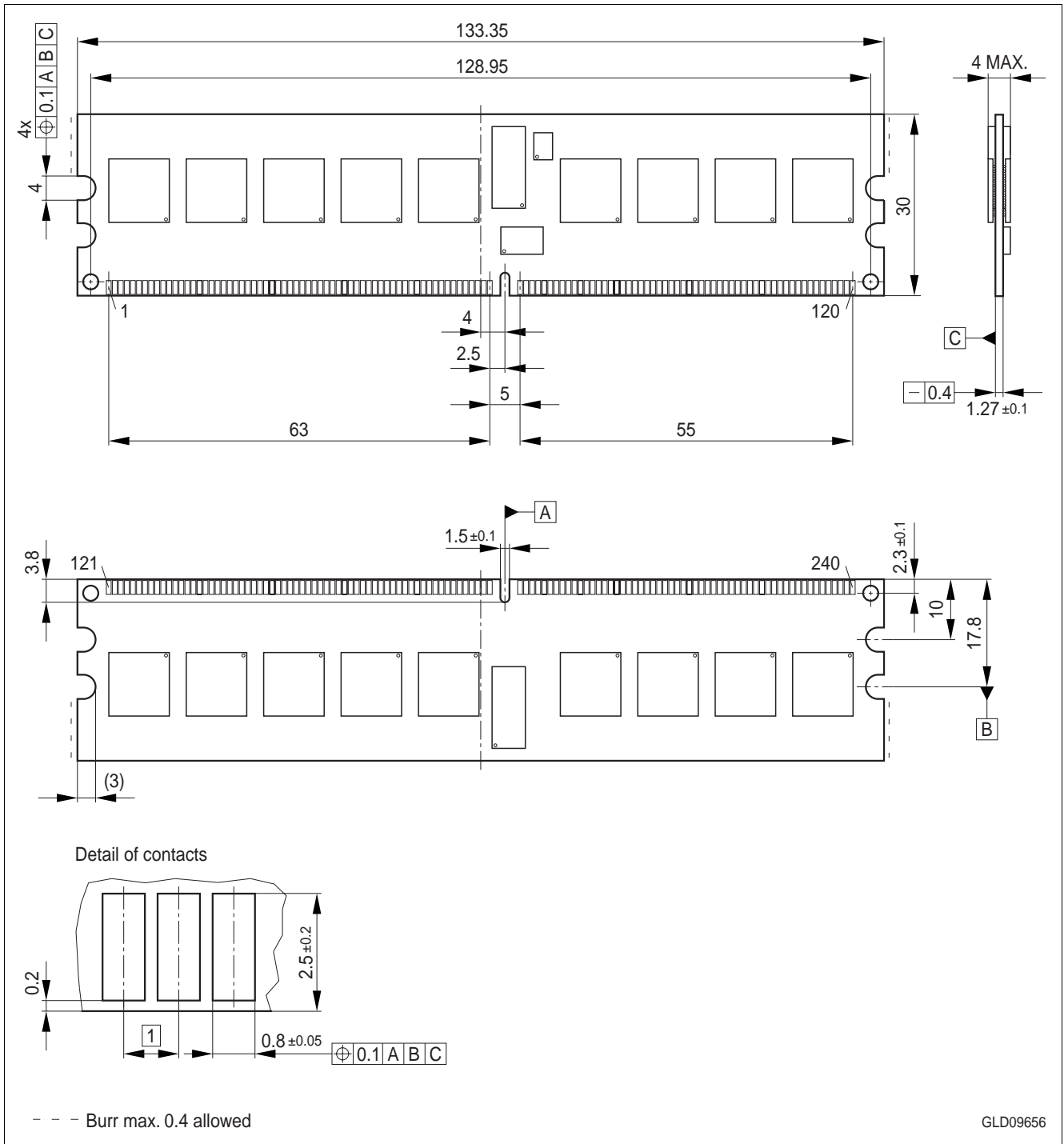
Figure 8 Package Outline Raw Card G L-DIM-240-12
