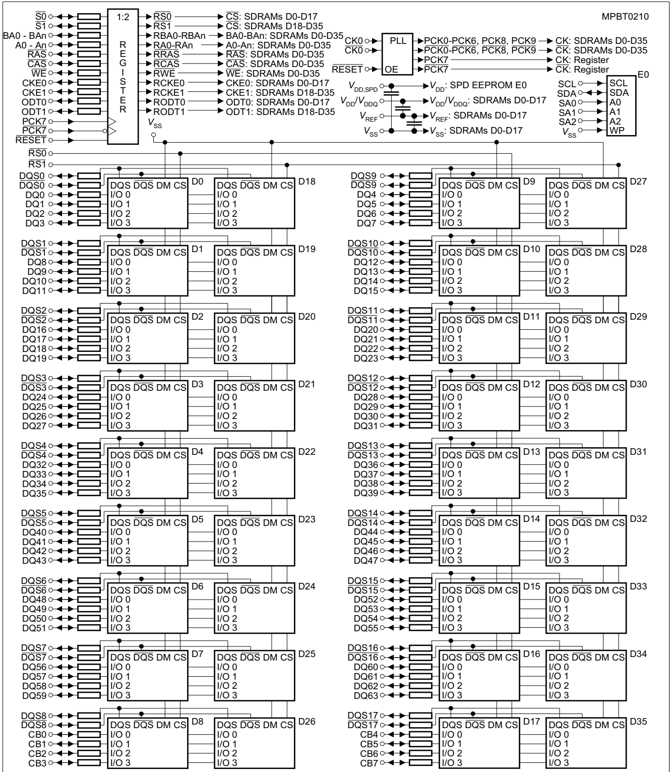
Figure 6 Block Diagram Raw Card L RDIMM (x72, 2Ranks, x4)
